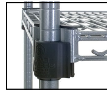
channel of shelf corner fits into slot of collar attached to split sleeve
