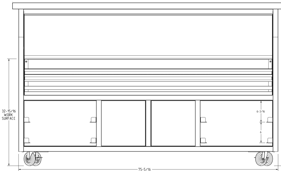
FRONT VIEW (WORKER'S SIDE)
