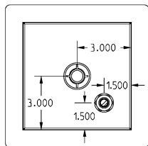
CUTOUT DIMENSIONS (width x length) 6 1/4" x 6 1/4" (159 x 159mm)
