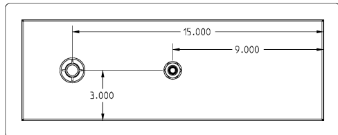
CUTOUT DIMENSIONS (width x length) 6 1/4" x 18 1/4" (159 x 464mm)
