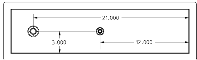
CUTOUT DIMENSIONS (width x length) 6 1/4" x 24 1/4" (159 x 616mm)
