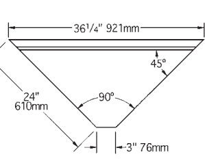
#MF90-22 Front Filler
