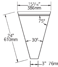
#MF30-22 Front Filler
