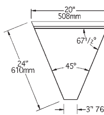
#MF45-22 Front Filler
