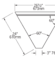
#MF60-22 Front Filler
