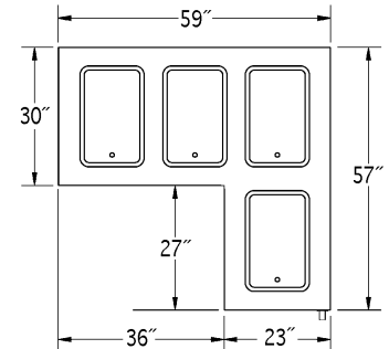
TOP VIEW OF #DCS4-TMLR
