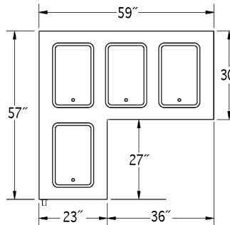
TOP VIEW OF #DCS4-TMLL
