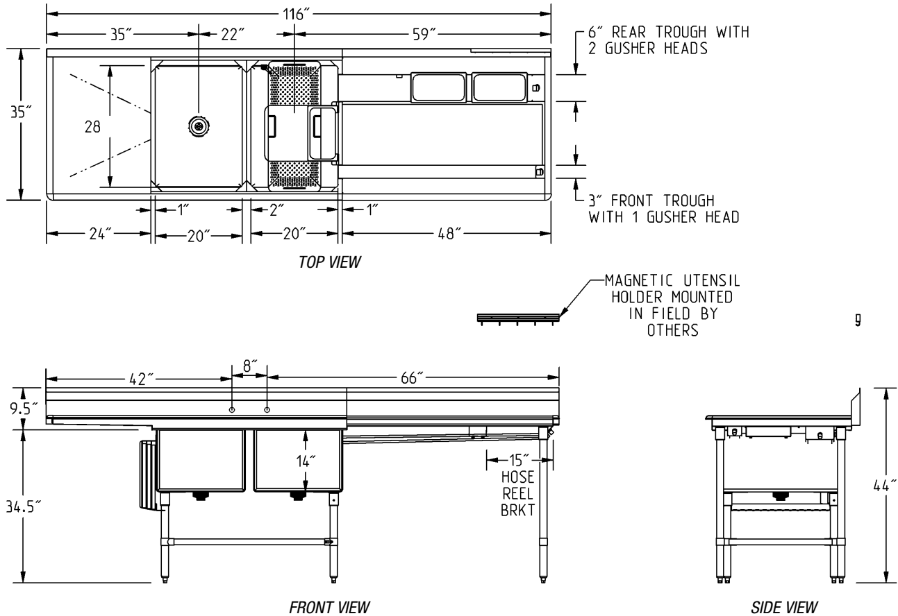
(model #FNP2840-2-24L-48TR shown)
