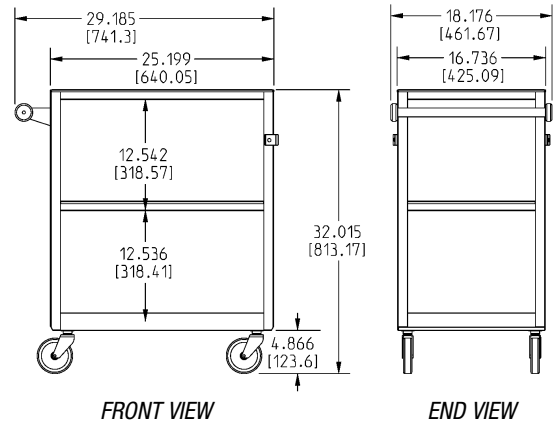
(CART WITH UPTURNS ON ALL SIDES OF ALL SHELVES SHOWN)
