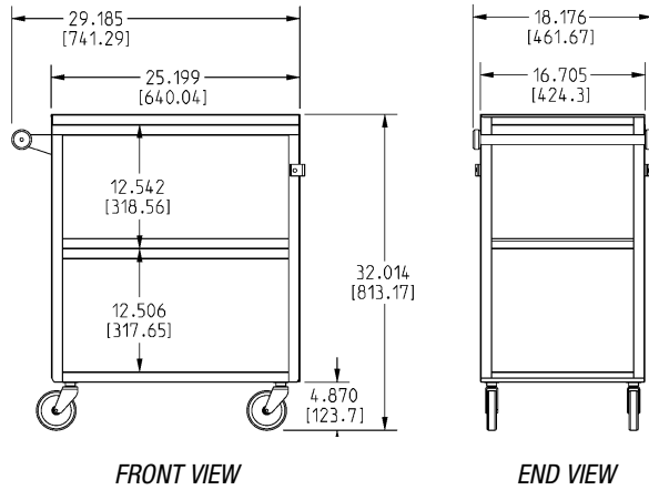
(CART WITH STANDARD UPTURNS SHOWN)
