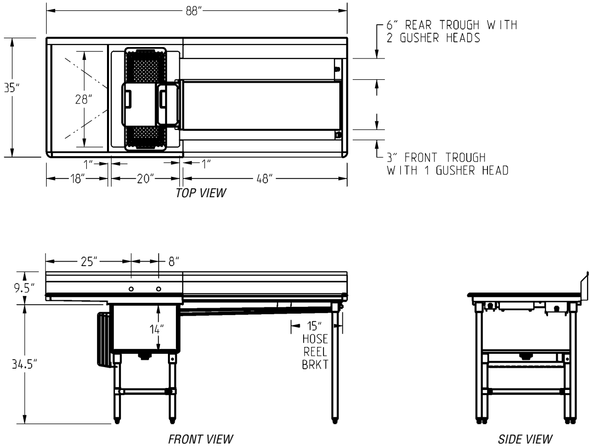
(model #FNP2820-1-18L-48TR shown)
