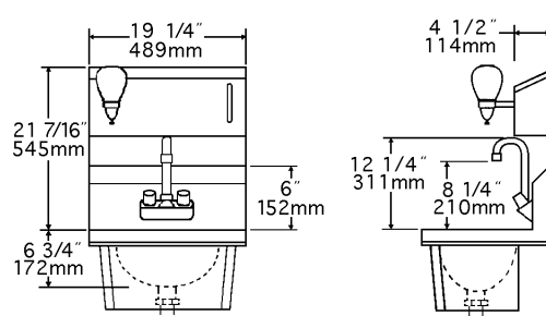
HSA-10-FDPS
