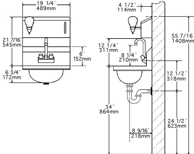
HSA-10-FDP
