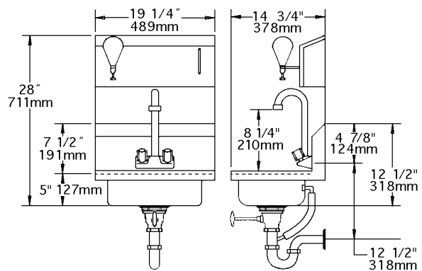
HSA-10-FODP
